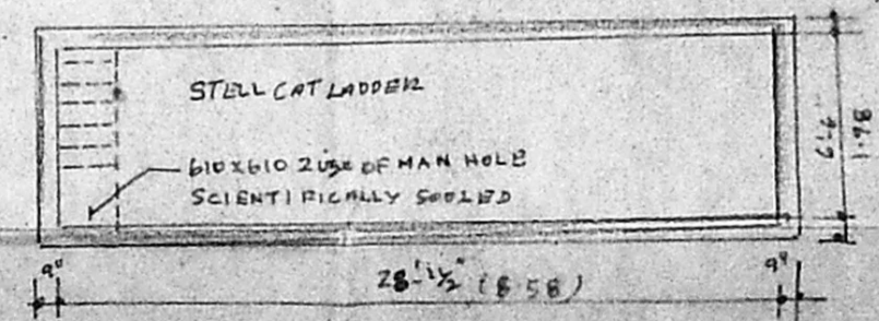
DETAILS OF SUMP
