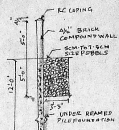
DETAILS OF PEBBLE BED
