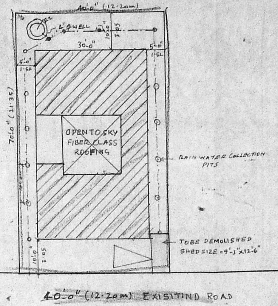
SITE PLAN
