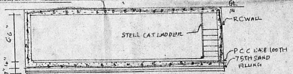
SECTION B-B1
